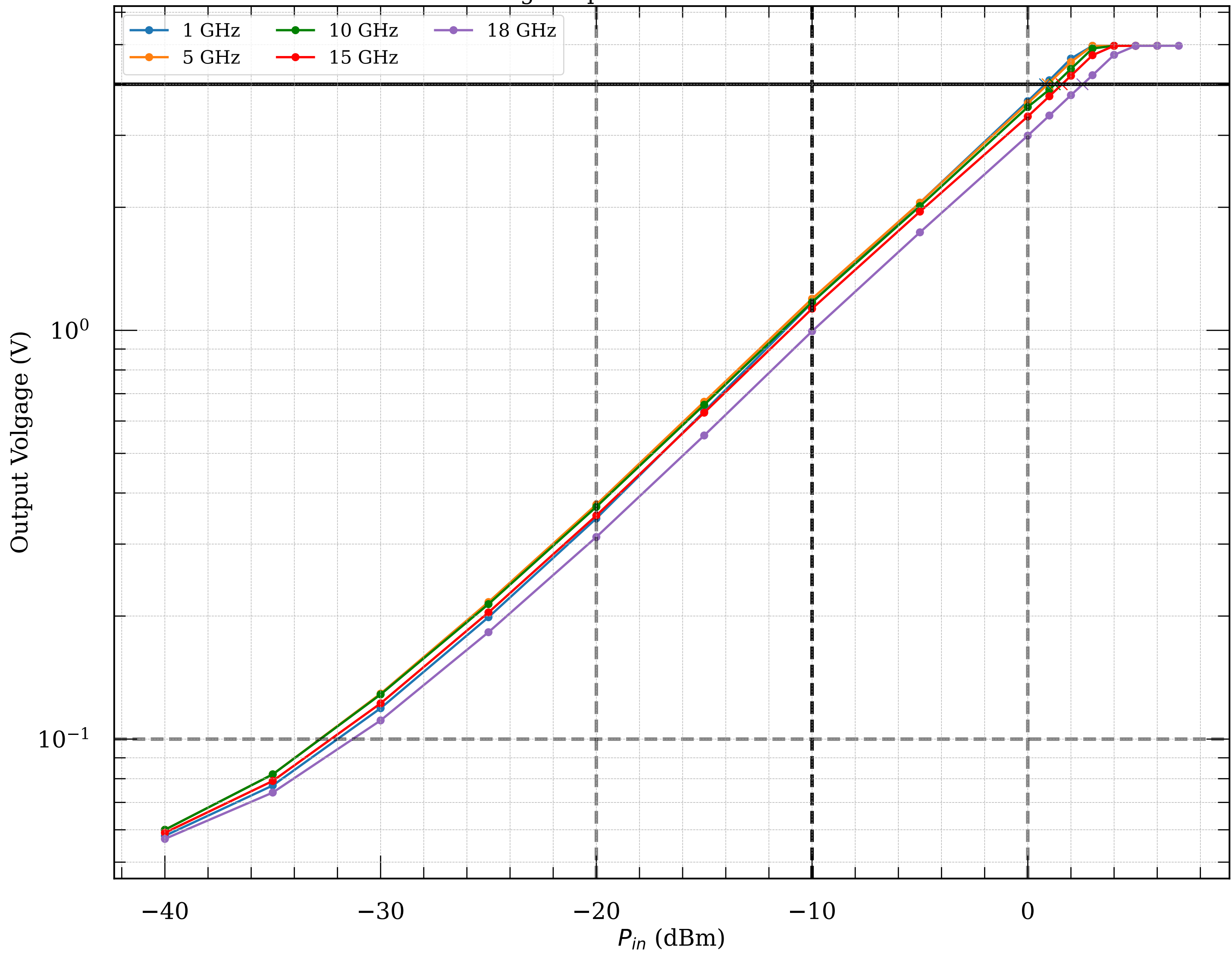
Measured voltage-to-power curve of detector module073
